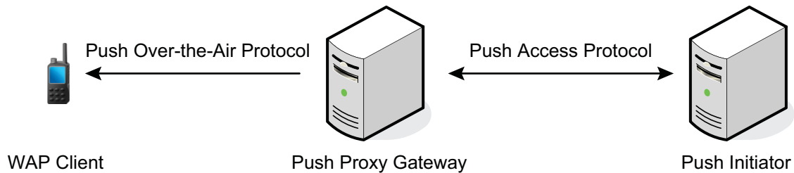
Figure 13: Push Framework
