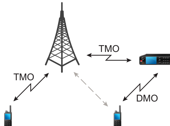
Figure 7: Communication Through Gateways
